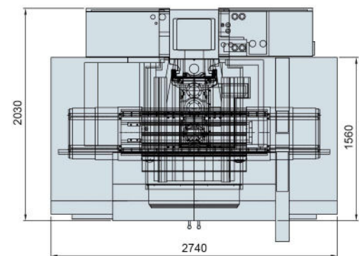
Top View (floor space required)
