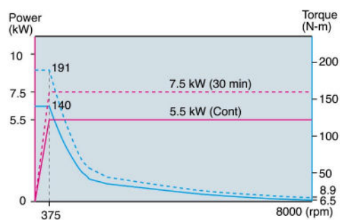
VMC-850 / 1050
